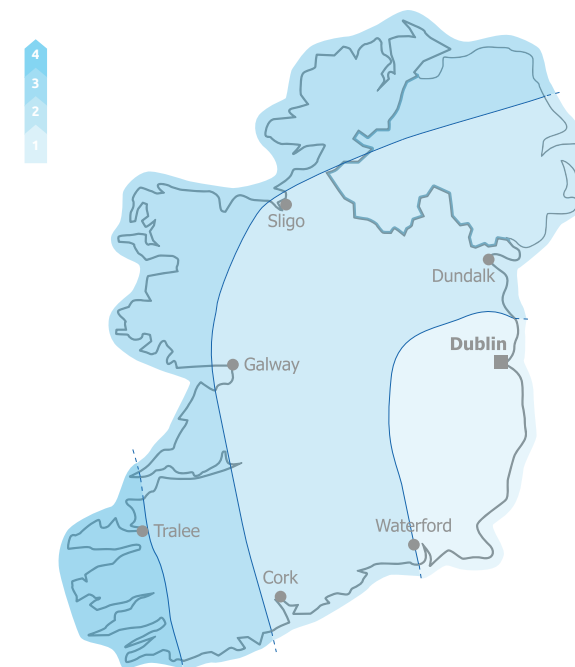
Fig. 2 - Wind map for Ireland
