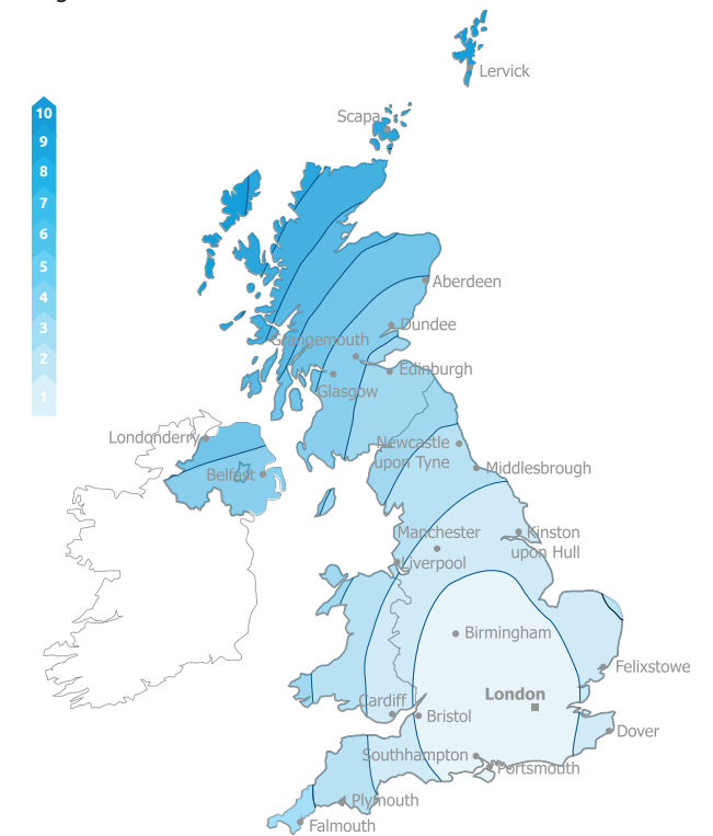
Fig. 1 - Wind map for United Kingdom
