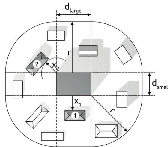
Figure 9. Influence of a high rise building on two neighbouring structures (based on EN 1991-1-4, Figure A.4)
