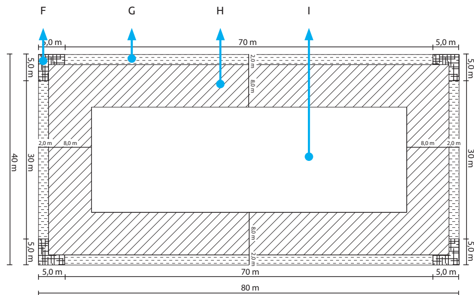
Figure 12. Example of flat roof zone designation
