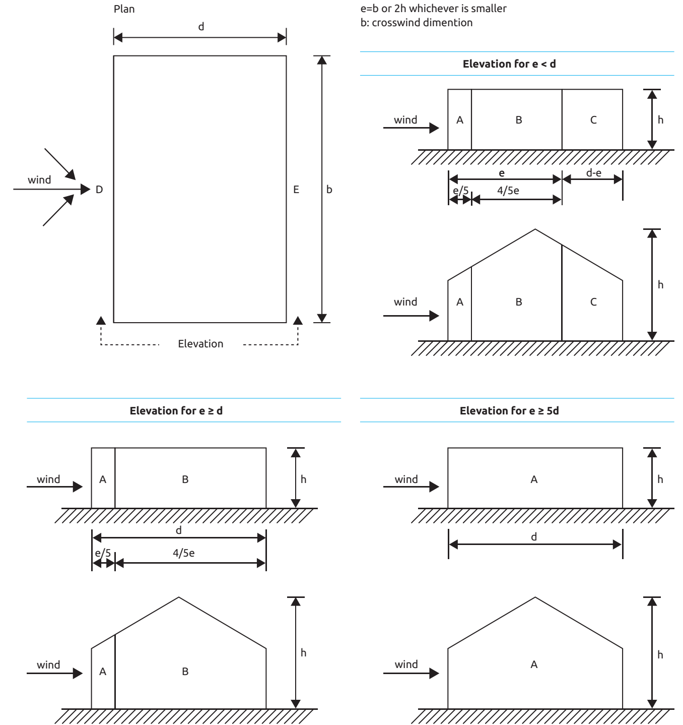
Figure 10.1 - Key for vertical walls
