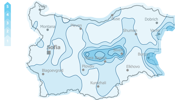
Fig. 6 - Wind map for Bulgaria
