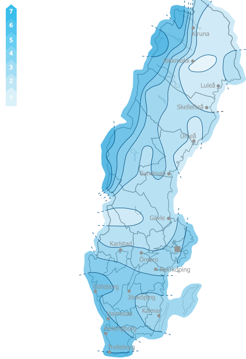
Fig. 4 - Wind map for Sweden
