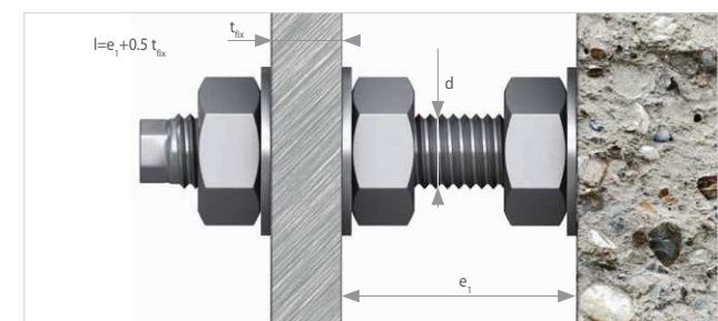
stand-off installation
