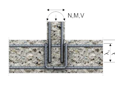
Figure 2 Overlap joint at a foundation of a column or wall where the rebars are stressed in tension
