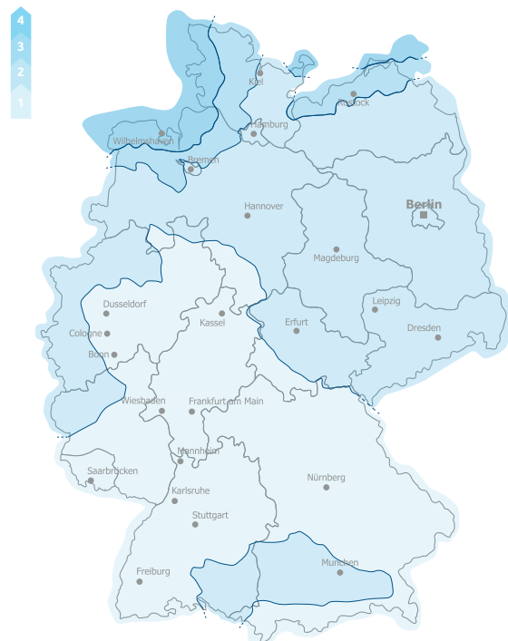
Fig. 7 - Wind map for Germany
