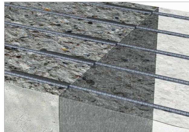
Figure 1.2: Overlap splice
