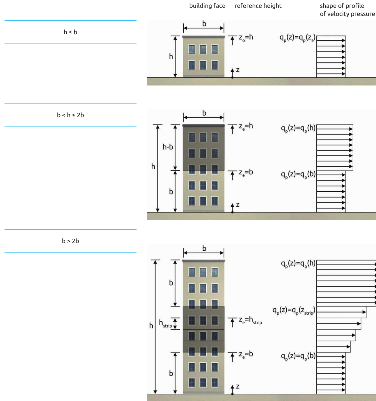
Figure 10 - Reference height, z_e , depending on hand b , and corresponding velocity pressure profile
