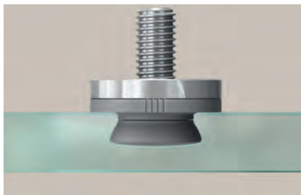
Glass point holder in single layered glass panels
